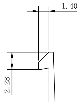
DETAIL B SCALE 4:1
